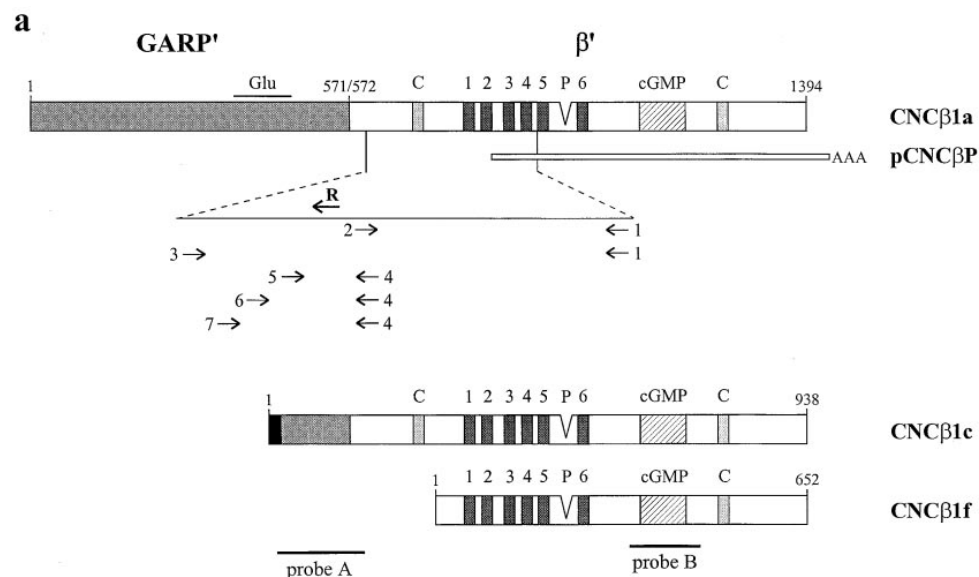
Figure 1. Cloning of \beta subunits and Northern blot analysis. (a) Schematic drawing of the primary structure of \beta subunits from bovine rod photoreceptor (CNC \beta 1a) and testis (CNC \beta 1c, CNC \beta 1f). CNC \beta 1a consists of a GARP part (aa 1–571) and a \beta' part (aa 572–1394). The GARP part is almost identical to the bovine GARP (Sugimoto et al., 1991). Glu refers to the glutamic acid-rich region; the transmembrane segments 1–6, the cGMP-binding site (cGMP), and the calmodulin-binding sites (C) are depicted as boxes. P, pore region. The different 5' ends of the long testis \beta subunits are represented as a black box. The COOH-terminal calmodulin-binding site does not modulate the channel activity (Grunwald et al., 1998; Weitz et al., 1998). The location of partial clone pCNC \beta P, and of riboprobes A and B used for Northern blot analysis is indicated. The location of primers 1–7 and primer R for 5' RACE is shown on a larger scale below the corresponding region of CNC \beta 1a. (b) Northern blot analysis of poly(A) + RNA from bovine testis (T) and retina (R). Probe A corresponding to aa 469–578 of CNC \beta 1a hybridized to transcripts of ~7.4 kb and to an ~4.4-kb transcript from retina and to an ~3.3-kb transcript from testis. Probe B corresponding to aa 909–1081 hybridized to transcripts of ~3.3 and 2.4 kb from testis and to an ~7.4-kb transcript from retina. Autoradiographic exposure was 3 d for testis samples and 12 h for
