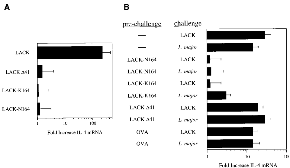
Figure 4. LACK analogue proteins fail to activate IL-4 mRNA in vivo. (A) Popliteal lymph node cells were collected 16 h after injection of 25 \mu g rLACK, LACK-K164, LACK-N164, or LACK \Delta 41 with the I-A d epitope deleted. RNA was purified and used to template a semiquantitative RT-PCR assay for the amounts of IL-4 transcripts. Results are expressed as the fold increase in IL-4 mRNA as compared with uninjected mice. Results shown represent comparable findings from three experiments. (B) BALB/c mice were injected in the hind footpads with 25 \mu g rLACK, LACK-K164, LACK-N164, LACK \Delta 41, or OVA (pre-challenge) and then again 24 h later with either 25 \mu g LACK antigen or 3 \times 10^6 L. major promastigotes (challenge). After 16 h, the popliteal lymph node cells were collected, RNA was isolated, and the relative
