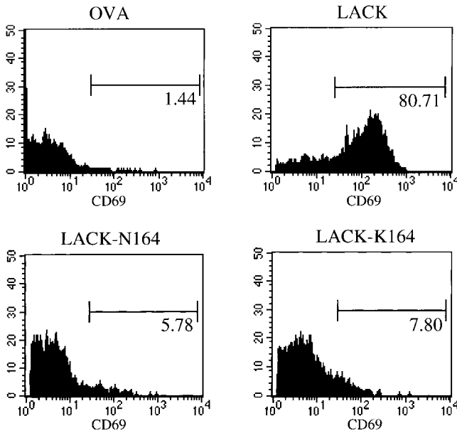
Figure 3. Activation of LACK-specific transgenic T cells in vivo by altered LACK proteins. Popliteal lymph node cells were collected from ABLT TCR- \alpha^0 mice that had been injected 24 h previously with 25 \mu g rLACK, LACK-N164, LACK-K164, or OVA proteins. Activation of V\beta 4^+ T cells was quantitated by the presence of the CD69 surface activation marker after gating on V\beta 4^+ T cells. Data are representative mice from three comparable experiments.
