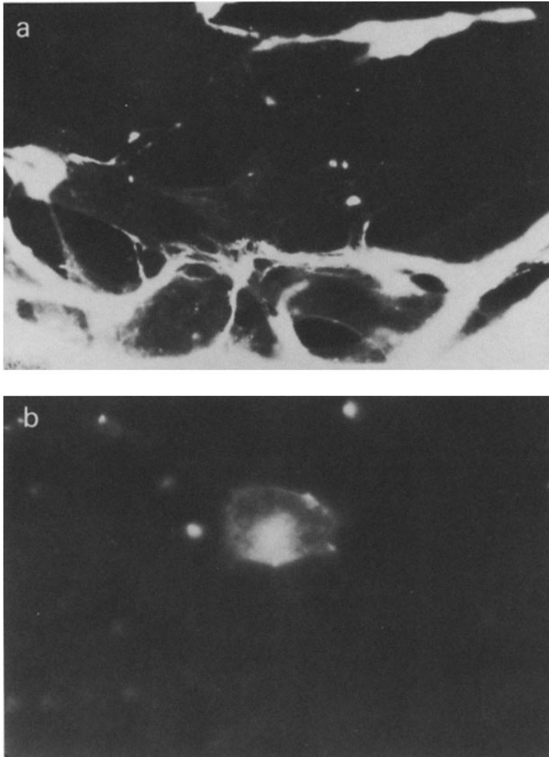
FIGURE 4 Fluorescence patterns of nearly confluent human fibroblasts containing fluorescent gangliosides. (a) Cultures incubated with rhodaminyl gangliosides ( 20 \mu\text{g/ml} ). (b) Same as in a except that cells were treated with trypsin.
