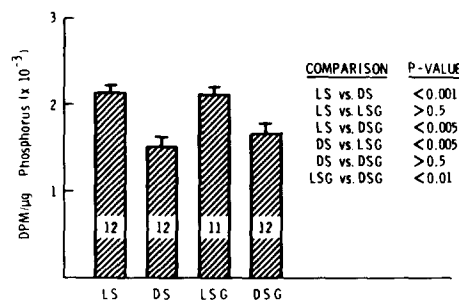
FIGURE 4 DPM of label incorporated per microgram of total lipid phosphorus of retinas preincubated for 15 min in the dark with 20\ \mu\text{M} strychnine, and then incubated for 2 h with [2\text{-}^3\text{H}] inositol in light (LS) or dark (DS) in the presence (LSG and DSG) or absence of 100\ \mu\text{M} glycine.
