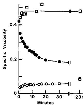
FIGURE 3 Viscometric assay of the dependence of the time course of nucleated actin polymerization on the concentrations of actin and profilin. (A) Dependence on the concentration of Acanthamoeba actin monomers. Conditions: 50 mM KCl, 0.28 mM ATP, 10 mM imidazole, pH 7.0 with 0.75 \mu M polymerized actin as nuclei. Concentrations of actin monomers are given beside each curve in micromoles per liter. (B) Effect of profilin on the time course of polymerization of 10 \mu M Acanthamoeba actin monomers nucleated with 0.75 \mu M polymerized actin in 50 mM KCl, as in A. The concentrations of profilin in micromoles per liter are given beside each curve. (C) Effect of profilin on the time course of polymerization of 10 \mu M Acanthamoeba actin monomers nucleated with 0.75 \mu M polymerized actin in 50 mM KCl, plus 1 mM MgCl 2 . The concentrations of profilin in micromoles per liter are given beside each curve. Inset : Profilin concentration dependence of the initial rates of nucleated viscosity change. Rates are expressed as fractions of the control without profilin. \circ , 10 \mu M Acanthamoeba actin in 50 mM KCl (control rate 0.17 cs/min); \Delta , 10 \mu M Acanthamoeba actin in 50 mM KCl, 1 mM MgCl 2 (control rate 0.23 cs/min); \square , 10 \mu M muscle actin in 50 mM KCl (control rate 0.13 cs/min). (D) Effect of profilin on the time course of polymerization of 10 \mu M muscle actin monomers nucleated with 0.75 \mu M polymerized actin in 50 mM KCl, as in A. The concentrations of profilin in micromoles per liter are given beside each curve.
