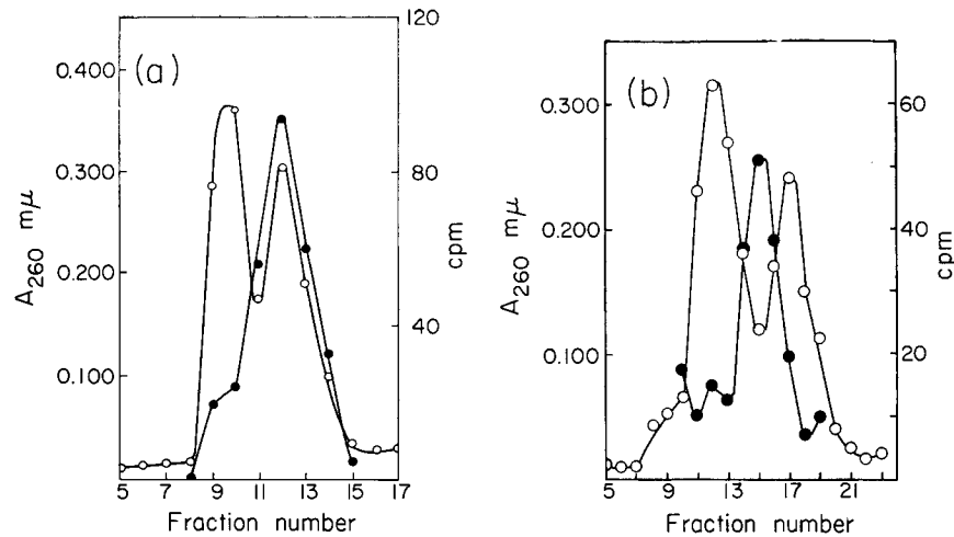
FIGURE 2 Hybridization of nRNA- 3 H from salivary glands of Rhynchosciara and of ribosomal RNA- 3 H from Xenopus laevis with CsCl fractionated DNA from Rhynchosciara . (a) 50 µg of salivary gland DNA was centrifuged in CsCl together with 50 µg of E. coli DNA, which was used as a marker (peak at left). Centrifugation was done in a rotor No. 40 (Spinco Division, Beckman Instruments, Fullerton, Calif.) at 42,000 rpm, for 34 hr at 15°C, according to conditions described by Flamm et al. (13). 22 fractions were collected, and those containing DNA were used for hybridization with 80 µg/ml nRNA- 3 H (280 cpm/µg), under the conditions described in Fig. 1. (b) 30 µg of Rhynchosciara ovary DNA was centrifuged in CsCl together with 50 µg of E. coli DNA. Centrifugation was done at 38,000 rpm for 46 hr at 15°C in rotor No. 40 (Spinco Division, Beckman Instruments). 25 fractions were collected, and those containing DNA were used for hybridization with 2 µg/ml rRNA- 3 H of Xenopus (20,000 cpm/µg) under the conditions described in Fig. 1, except that the time of annealing was 20 hr. (●—●), radioactivity in the hybrid; (○—○), absorbance at 260 mµ of the fractions.
