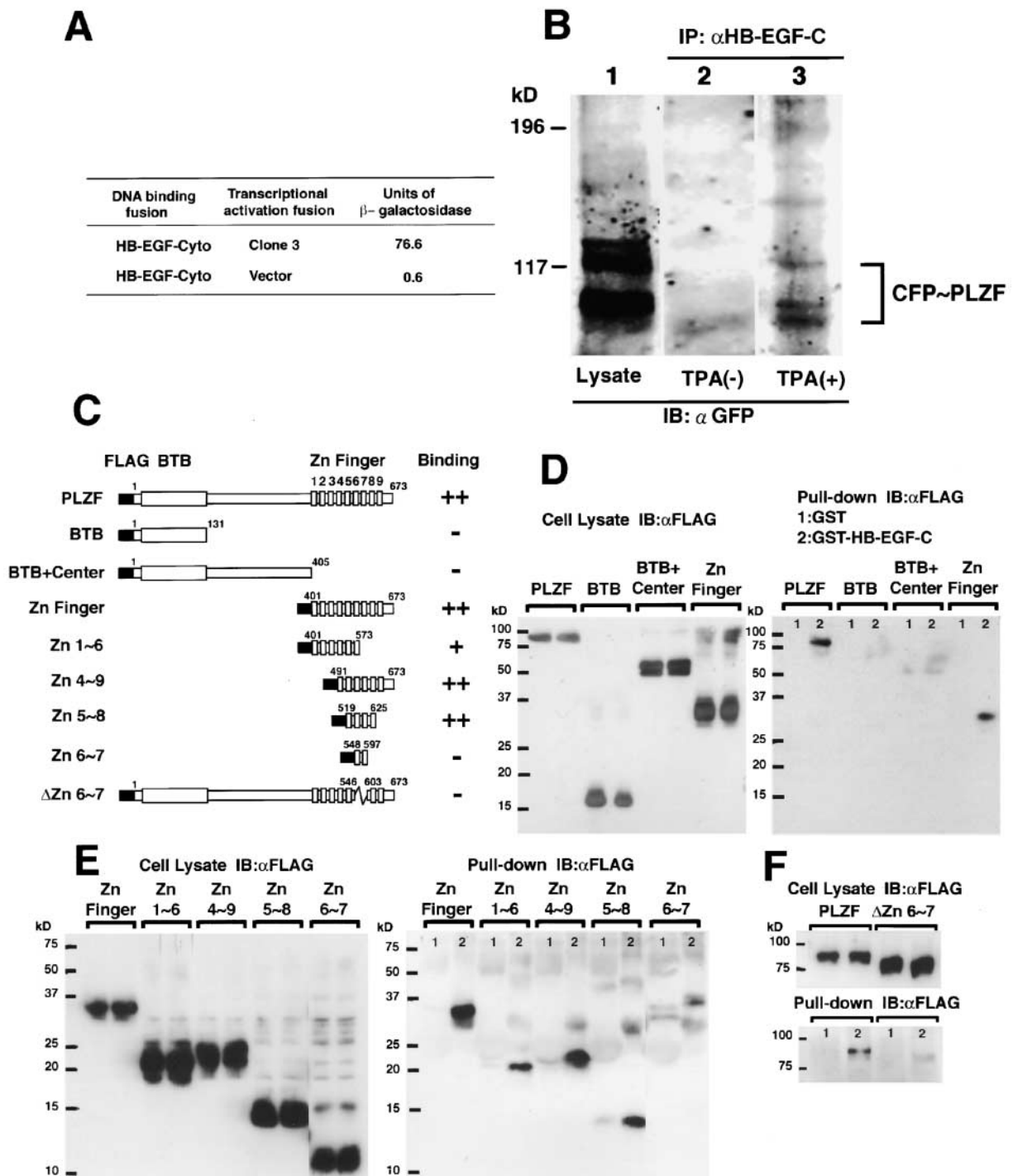
Figure 2. Identification of PLZF as an HB-EGF-C binding protein. (A) We used the yeast two-hybrid method and screened a human heart cDNA library with the cytoplasmic region of HB-EGF (HB-EGF-Cyto; residues 185–208) as bait. One of the positive clones (clone 3) was identified as encoding a portion of PLZF. (B) COS cells were transiently transfected with a proHB-EGF expression vector and a CFP-PLZF expression vector encoding a fusion protein in which CFP was fused to the amino terminus of PLZF, stimulated for 60 min with TPA, and lysed. Expression of CFP-PLZF was confirmed by immunoblotting of the whole lysate with anti-GFP antibody (lane 1). The lysates were immunoprecipitated with anti-HB-EGF-C antibody (#H1), and the precipitates were immunoblotted with anti-GFP antibody (lanes 2 and 3). Note that the interaction between PLZF and HB-EGF was observed when cells were stimulated with TPA. (C–F) GST pull-down assay. Cell lysates containing the FLAG-tagged PLZF derivatives were incubated with GST (1) or GST-HB-EGF-C (2) beads, and bound proteins were detected by immunoblotting using an anti-FLAG antibody (right). Expression of the derivatives was also confirmed by immunoblotting using an anti-FLAG antibody (left). (C) Schematic diagrams of FLAG-tagged PLZF derivatives. Nine zinc finger motifs in the PLZF protein are numbered from first to ninth. Binding properties of PLZF derivatives to GST-HB-EGF-C is summarized in the right lane of each structure. The binding properties are based on the estimation from the intensity of bands as compared with the control band and are indicated as ++ (>50%), + (50–10%), and - (<10%). (D) Full-length PLZF and the fragment containing nine zinc finger motifs (Zn Finger) were bound to GST-HB-EGF-C, but not to GST alone. (E) The fragments consisting of zinc finger motifs 4~9 (Zn4~9) and 5~8 (Zn5~8) were bound to GST-HB-EGF-C stronger than the fragment with zinc finger motifs 1~6 (Zn1~6). The fragment consisting of zinc finger motifs 6~7 (Zn6~7) was not efficient for the interaction. (F) Deletion mutant ( \Delta Zn6~7) showed that the region with Zn6~7 was essential for HB-EGF-C-PLZF interaction.
