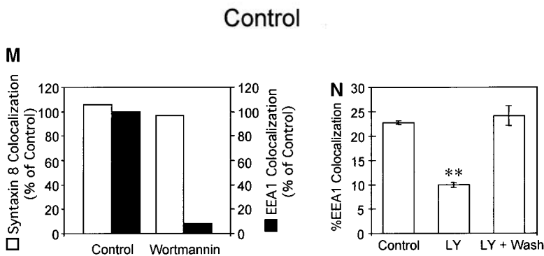
colocalization of latex beads and Syntaxin 8 staining. Cells containing nascent phagosomes (10 min of phagocytosis) were treated with medium alone (A, B, C, and F), 100 nM wortmannin (D, E, I, and L), exposed continuously to 200 \mu M LY294002 (20 min) (G and H), or first treated with LY294002 for 10 min, which was then removed by washing, and incubated for an additional 10 min in medium without the inhibitor (J and K) as described in Materials and methods. (M) ■, Quantitation of EEA1 colocalization with phagosomes (20 min after infection) in wortmannin treated and control cells; □, quantitation of staining with Syntaxin 8 ( n = 1,068 ; all samples). (N) Quantitation of EEA1 colocalization with phagosomes (30 min after infection) in control cells and LY294002-treated cells ( n = 1,816 phagosomes). The data are means \pm SE of three separate experiments. ** P = 0.0003 .
