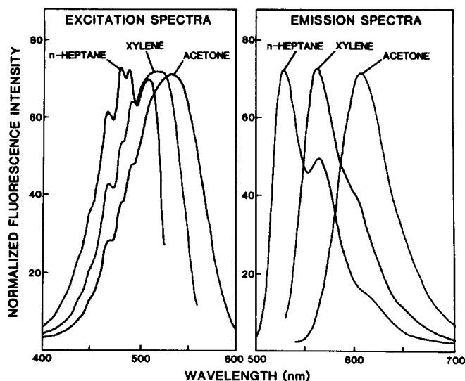
FIGURE 2 Excitation and emission fluorescence spectra of Nile red in n -heptane, xylene, and acetone. A 1 \mu g/ml solution of Nile red in each solvent was used. The excitation and emission spectra of Nile red were recorded at their corresponding emission or excitation maxima.
