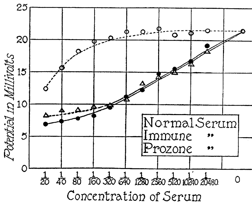
FIG. 1. Effect of unheated agglutinative, and heated agglutinative (inhibition zone) typhoid serum, and of normal serum upon P.D. and agglutination of B. typhosus . Solid line indicates agglutination; broken line, no agglutination. Experiment in G. P. A. buffer mixture, pH 7.0.
