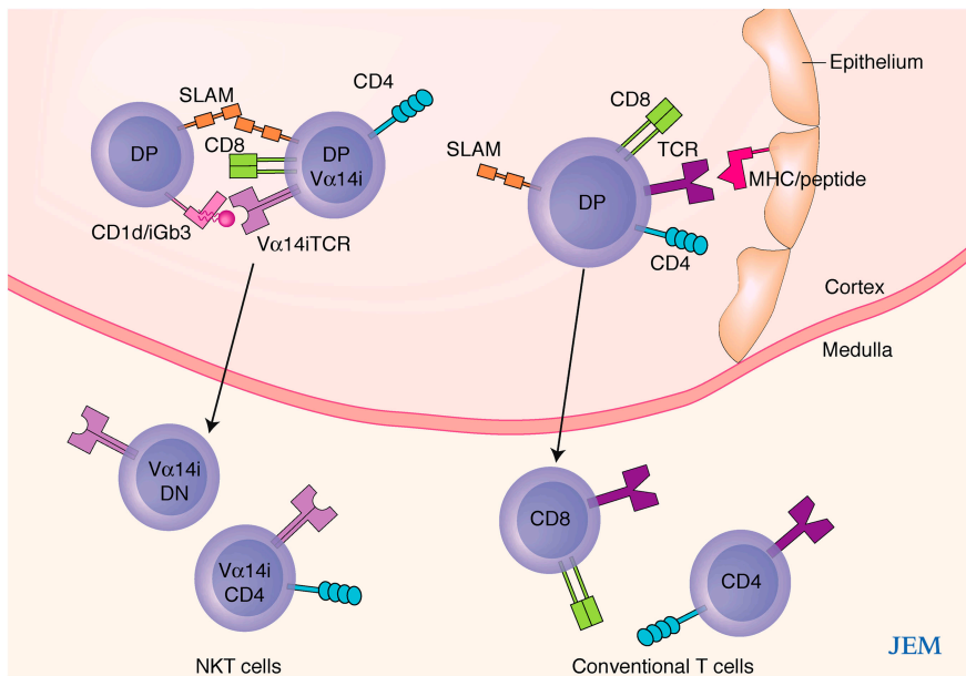
Figure 1. Potential scheme of SAP-dependent NKT cell selection. Homotypic interactions between V\alpha 14i TCR + and CD1d/iGb3 + cortical CD4 + CD8 + double positive (DP) thymocytes allow simultaneous SAP-dependent homotypic interactions between unidentified SLAM family members. Interactions between CD8 and CD1d might also occur. Heterotypic interactions between conventional (non- V\alpha 14i ) TCR + DP thymocytes and MHC-peptide + thymic epithelial cells allow CD8-MHC class I interactions.
