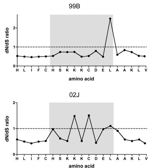
Figure 3. dN/dS values of acute subjects 99B and 02J. Analysis of dN/dS values suggests selective pressure at position 9 in the targeted B8-1395 epitope (shaded area) in subject 99B and positions 4, 6, and 9 in subject 02J (ratio > 1; dotted line). The residues are labeled with amino acids represented in the H77 reference sequence. ML phylogenetic trees were estimated by using the PAUP* package and dN/dS values were calculated using the CODEML program.
