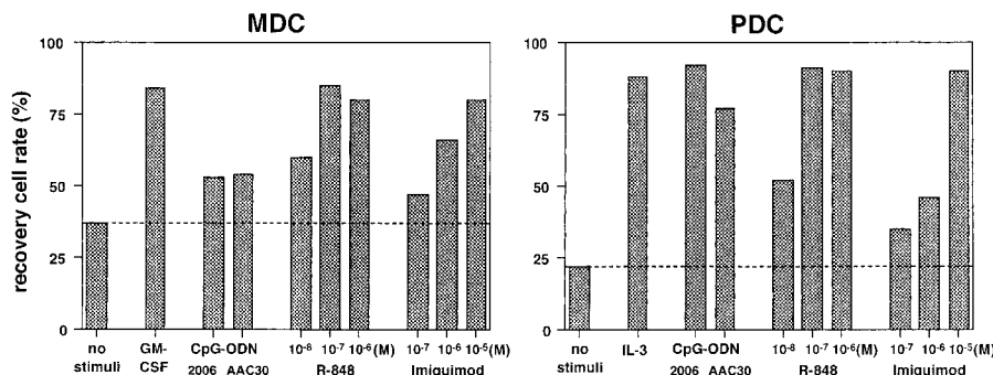
Figure 2. TLR-7 ligands enhance the survival of both MDCs and PDCs. MDCs and PDCs were incubated for 24 h with various stimuli. The viable cells in each DC subset were evaluated as annexin V-negative fractions by flow cytometry. The results are representative of three independent experiments.
