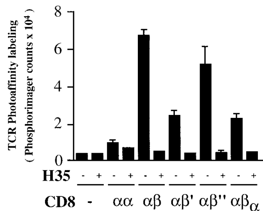
Figure 5. The cytoplasmic tail of CD8 \beta is required for efficient CD8-mediated increase in TCR photoaffinity labeling. T1.4 hybridoma cells ( 5 \times 10^6 /ml) with the indicated CD8 expression were incubated for 2 h at 0–4°C with soluble monomeric K d - 125 IASA''-YIPSAEK(ABA)I ( 2-6 \times 10^6 cpm/ml) in the absence or presence of anti-CD8 \beta mAb H35-17 (10 \mu g/ml). After UV irradiation cells were lysed in RIPA buffer, TCR immunoprecipitated, and analyzed by SDS-PAGE and PhosphorImaging. Mean values and SD were calculated from six experiments.
