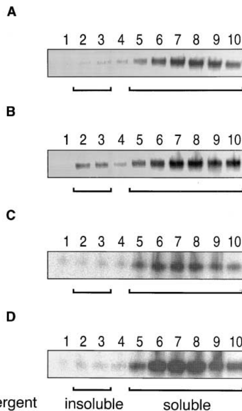
Figure 7. CD8 \alpha\beta mediates raft association of TCR/CD3. T1.4 hybridomas ( 5 \times 10^7 ) expressing no CD8 (A), CD8 \alpha\beta (B), CD8 \alpha\beta' (C), or CD8 \alpha\beta'' (D) were photoaffinity labeled at 26°C with K d - 125 IASA"-YIPSAEK(ABA)I (0.5–1.5 \times 10^8 cpm/7 ml). After UV irradiation the washed cells were lysed in 0.5% Brij58 and the lysates fractionated on sucrose density gradients. Fractions were collected from the top and immunoprecipitated with anti-TCRC \beta mAb H57. The immunoprecipitates were analyzed by SDS-PAGE and PhosphorImaging.
