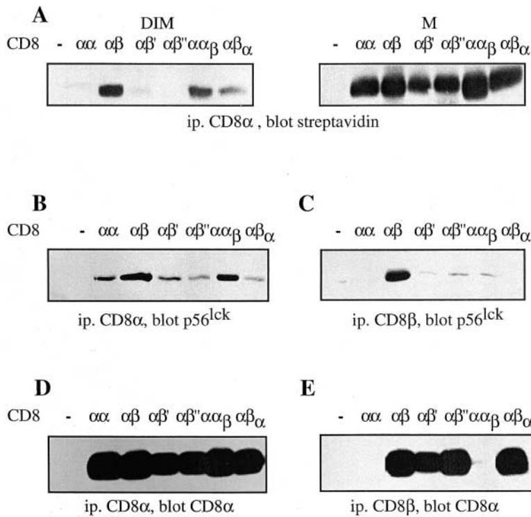
Figure 4. Palmitoylation of CD8 \beta is essential for CD8 localization in rafts and efficient lck association. (A) T1.4 hybridomas with the indicated CD8 expression were surface-biotinylated, lysed in cold TX-100 (1%), and fractionated in M and DIM fractions. These were immunoprecipitated with anti-CD8 \alpha mAb 53.6.72. The samples were analyzed by SDS-PAGE and Western blotting with streptavidin. (B–E) T1.4 hybridomas with the indicated CD8 expression were lysed in Brij96 (1%) and the lysates immunoprecipitated with mAb 53.6.72 (B and D) or anti-CD8 \beta mAb H35-17 (C and E). The immunoprecipitates were analyzed by SDS-PAGE and Western blotting with anti-lck mAb 3A5 (B and C) or anti-CD8 \alpha antiserum (D and E). Note that anti-CD8 \beta mAb H35 is unable to precipitate CD8 \alpha\alpha and CD8 \alpha\beta . One out of two experiments is shown.
