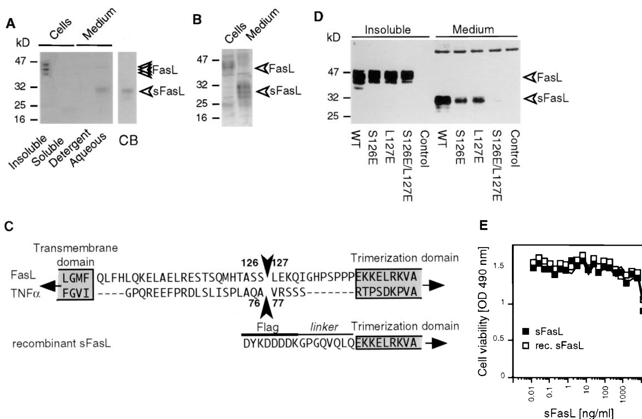
Figure 1. Recombinant and naturally processed sFasLs show marginal apoptotic activity on human cells. (A) Processing of membrane-bound FasL to sFasL. Cellular extracts of a 293 cell clone stably transfected with human FasL cDNA, were separated into Triton X-114-insoluble ( Insoluble ) and -soluble ( Soluble ) fractions. Cell supernatants ( Medium ) were separated into detergent and aqueous fractions by Triton X-114 phase separation. Samples were analyzed by Western blotting for the presence of FasL using an antibody specific for the extracellular segment of the ligand. The indicated FasL and sFasL bands were absent in mock transfected controls (D, and data not shown). The processed sFasL was purified by Fas/Fc affinity chromatography and visualized by Coomassie blue staining (CB). (B) 293 cells were transfected with mouse FasL cDNA. Total, unfractionated cellular extracts and cell supernatants were analyzed by Western blotting as described for A. (C) Site of proteinase-induced cleavage of FasL. Metalloproteinase(s) present in 293 cells cleave(s) membrane-bound FasL at the Ser126–Leu127 bond, liberating a soluble form of FasL. The cleavage site of the TNF- \alpha precursor is shown for comparison. (D) The effect of cleavage site mutations on FasL processing. Wild-type (WT) FasL as well as FasL mutated at the P1 site (S126E), at the P1' site (L127E), and at both the P1 and P1' sites (S126E/L127E) were transiently transfected into 293T cells. Insoluble proteins (containing membrane-associated FasL) and medium (containing processed sFasL) were analyzed by Western blotting as described above. To achieve similar loading of soluble and cell-associated FasL, the supernatants corresponding to 10 times more cells were loaded on the gel. A nonspecific band at 60 kD indicates equal loading of the gel. In the control lane, cell extracts of nontransfected 293 cells were analyzed. (E) Activity of naturally processed ( open squares ) and recombinant ( closed squares ) sFasL on Jurkat T cells.
