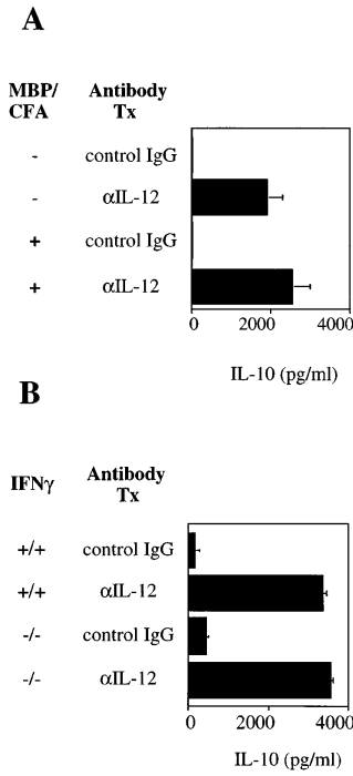
Figure 4. Suppression of IL-10 production by endogenous IL-12 is antigen and IFN- \gamma independent. (A) Splens were harvested from naive or MBP 87-106 -primed SJL mice that had been injected with anti-IL-12 or control IgG on days -10, -6, and -3 before killing. Supernatants were assayed for IL-10 after 96 h of culture. Results represent the means of four independent experiments with groups consisting of 5-7 mice in each experiment. Standard deviations reflect the variability between individual experiments. (B) Naive C57BL/6 wild-type and IFN- \gamma -/- mice were treated as in A. Results represent the means and standard deviations of two independent experiments in which splens were pooled from four mice in each group.
