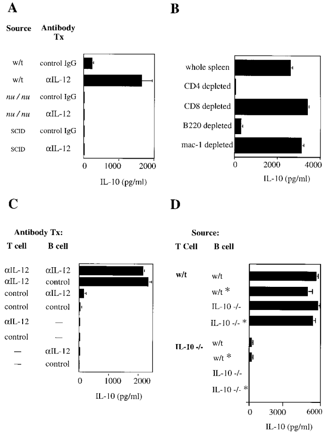
Figure 5. After neutralization of IL-12, IL-10 is produced by antigen nonspecific CD4 + T cells in collaboration with B cells. Splens were harvested from unimmunized mice that had been injected intraperitoneally with 0.5 mg of control IgG or anti-IL-12 on days -10, -6, and -3 before killing. Supernatants were collected for assay of IL-10 after 96-120 h of culture. (A) IL-10 production by splenocytes from BALB/c wild-type ( w/t ), nu/nu , and SCID mice at 96 h. Results represent means and standard deviations of two independent experiments in which splens were pooled from 3-5 mice in each group in each experiment. (B) Splenocytes from anti-IL-12 treated SJL mice ( n = 5-6 ) were depleted of various subpopulations using sheep anti-fluorescein biomag beads and FITC-conjugated mAbs specific for the cell surface markers indicated. Recovered cells ( 4 \times 10^6 cells/ml) from each group were cultured and supernatants assayed for IL-10 after 120 h. In each case, the recovered cells were 99-100% free of the depleted population as determined by flow cytometry using PE-conjugated mAbs (not shown). Results represent means and standard deviations of three independent experiments. Whole spleen and subpopulation preparations derived from control IgG-treated donors failed to produce detectable IL-10 (not shown). (C) CD4 + T cells and B220 + B cells purified from splens of anti-IL-12 or control IgG-treated SJL mice ( n = 4-7 /group) were cocultured ( 2 \times 10^5 of each in 200 \mu l) in 96-well microtiter plates. Supernatants were collected at 120 h to quantify IL-10 levels. Results represent means and standard deviations of four independent experiments. Levels of purity ranged from 90 to 95% for CD4 + T cells and 93-98% for B220 + B cells as assessed by flow cytometry (not shown). (D) CD4 + T cells from splens of anti-IL-12-treated C57BL/10 wild-type or IL-10 -/- mice were cocultured with B220 + B cells purified from splens of either anti-IL-12 or control IgG-treated donors ( 2 \times 10^5 of each in 200 \mu l). An asterisk (*) denotes B cells taken from anti-IL-12-treated mice. Supernatants were collected at 144 h to quantify IL-10 levels. Results represent means and standard deviations of two independent experiments. Levels of purity ranged from 92 to 94% for CD4 + T cells and from 95 to 99% for B220 + B cells. Three to five donor mice were used for each group in each experiment. CD4 + T cells purified from control IgG-treated donors failed to produce IL-10 irrespective of the B cells with which they were combined (not shown).
