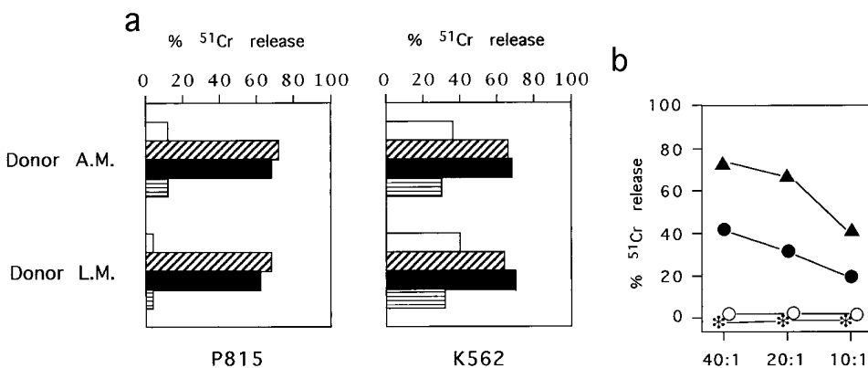
Figure 6. p46-mediated triggering of cytolytic activity in fresh peripheral blood NK cells. (a) Freshly isolated peripheral blood NK cells were analyzed for their ability to kill the indicated Fc\gamma R^+ target cells in the absence of mAb ( \square ) or presence of anti-CD16 ( \boxplus ), BAB281 ( \blacksquare ), or anti-CD56 mAb ( \square ). The effector target ratio was 20:1 against P815 target cells and 10:1 against K562 target cells. (b) Freshly isolated PBL were sorted according to the lack of expression of p46 ( \circ ) or CD3 ( \blacktriangle ) or both p46 and CD3 ( \bullet ) and compared to unfractionated cells ( \bullet ) for cytolytic activity against ^{51}Cr -labeled K562 target cells in the absence of added mAbs.
