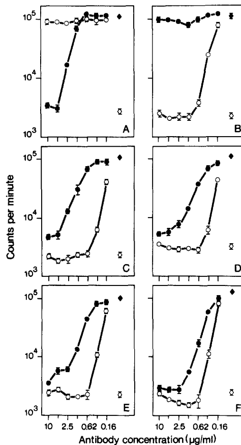
Figure 1. mAbs specific for \text{A}\beta^d and \text{E}\alpha block the T cell response of T cell hybridomas specific for peptide 110-121. T cell hybridomas were stimulated with SpW Mb presented by A20 cells in the presence of serial twofold dilutions of the \text{A}\beta^d -specific antibody MKD6 (●) or the \text{E}\alpha -specific antibody 14.4.4S (○); control wells contained medium alone (◇) or antigen without antibody (◆). Hybridomas were: (A) 11.12.8b-H5.1; (B) 13.26.8-H6.1; (C) 8.2.1d-Ha1.5; (D) 9.4.23.H1b.2; (E) 11.3.7e-H2.2.3; and (F) 12.2.9-H7.2. Those hybridomas are subclones of those in Fig. 2 and Table 1. Antigen concentrations, chosen to give slightly suboptimal proliferation, were 0.16 \mu\text{M} (B and C), 0.31 \mu\text{M} (A and E), 0.62 \mu\text{M} (F), or 1.25 \mu\text{M} (D). Results are given as the mean of triplicate wells \pm SE.
