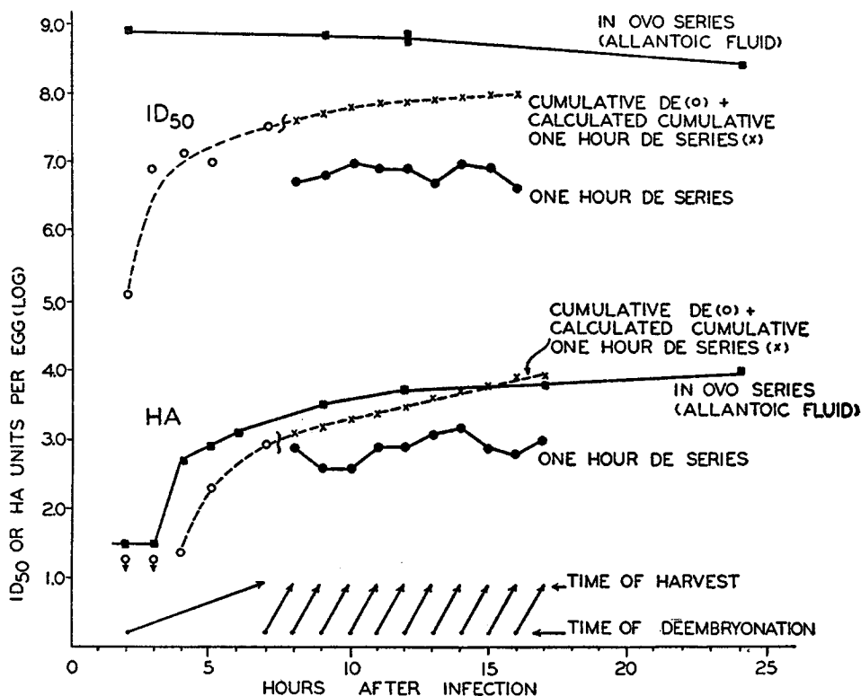
FIG. 6. Experiment 4. The yields of ID 50 and HA units from eggs deembryonated at hourly intervals (7th to 16th hour) after infection with 10^{9.6} ID 50 and incubated for 1 hour thereafter, (1 hour DE series) and comparison of the calculated cumulative yields derived from these values with the yields obtained in intact chick embryos.
