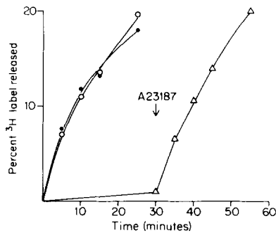
FIGURE 7 Effect of K^+ on A23187 induced release of 20:4. Cells were isolated, labeled, washed, overlaid with high K^+ (O) or high Na^+ medium (●), and challenged with the ionophore A23187 (10 \mu g/ml). At the times indicated duplicate aliquots of medium were removed and counted. After 25 min, the cells were washed, scraped into Triton X-100 and the radiolabel and protein content of the cell lysates was quantitated. Cells were also preincubated for 30 min in high K^+ medium ( \Delta ), treated with A23187, and the time course of ^3H -20:4 release was assessed. Values are expressed as percent of total cellular 20:4 released into the medium and are the mean of triplicate cultures.
