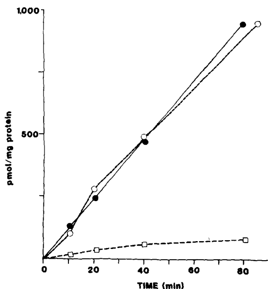
FIGURE 3 Tyrosine-specific phosphorylation of angiotensin II by VSV-associated protein kinase. Purified VSV was incubated in a reaction containing [ \gamma - ^{32}\text{P} ]ATP and angiotensin II as substrate (see Materials and Methods). The ^{32}\text{P} -labeled angiotensin in the product was fractionated by paper electrophoresis and quantitated by Cerenkov counting. The activity was quantitated as picomole of phosphate transferred per milligram of VSV protein. (□) VSV grown in BHK control cells; (●) VSV grown in BHK suspension cells; (○) VSV grown in RSV-transformed BHK cells.
