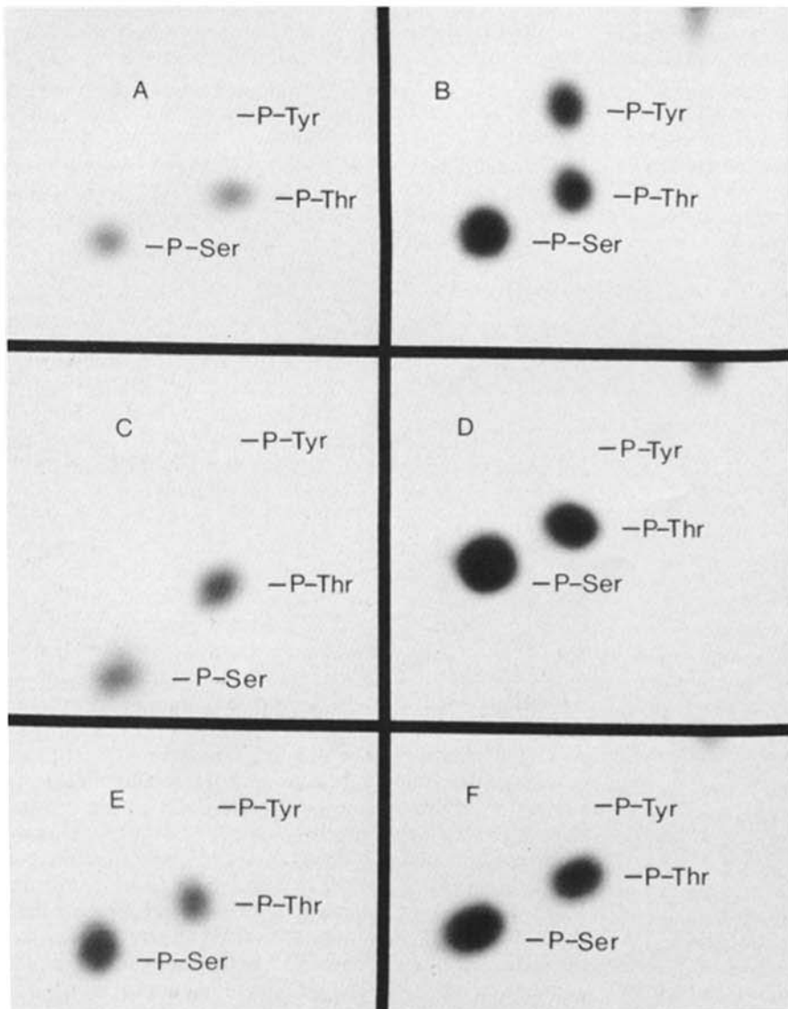
FIGURE 5 Amino acids phosphorylated by enzymes in detergent-soluble and -insoluble cell fractions. The detergent-soluble and -insoluble cell fractions from monolayer cultures were prepared as described in Materials and Methods. 12 \mu g of the detergent-soluble fraction of RSV-transformed BHK cells (A), control BHK cells (C), BHK suspension cells (E), and an equivalent proportion of the detergent-insoluble fraction from the RSV-transformed BHK cells (B), control BHK cells (D), and BHK suspension cells (F), were incubated in a reaction and ^{32} P-labeled phosphoamino acids were analyzed as described in Fig. 2.
