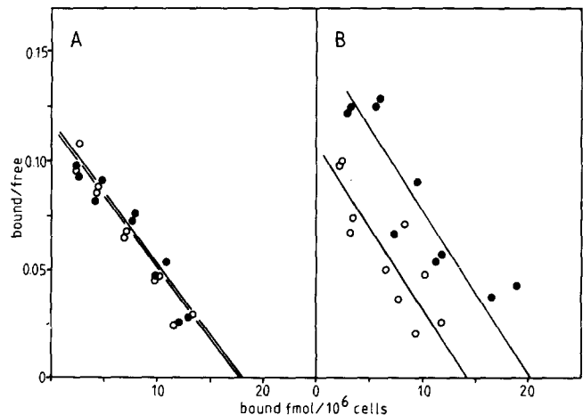
FIGURE 4 Energy dependence of the reappearance of \beta -adrenergic receptors. All cells were treated with 20 mM 2-deoxyglucose and 10 \mu\text{M} antimycin A with (O) or without (●) 1 \mu\text{M} l -isoproterenol. After extensive washing the cells were incubated for 90 min at 37^\circ\text{C} with CGP-12177 either in the absence (A) or in the presence (B) of 20 mM 2-deoxyglucose and 10 \mu\text{M} antimycin A.
