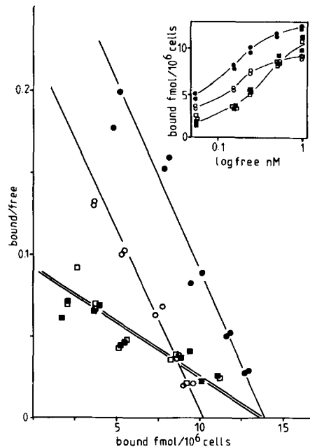
FIGURE 1 Reversible decrease of binding sites after isoproterenol treatment. Isoproterenol-pretreated (open symbols) or control cells (closed symbols) were incubated with [ ^3 H]CGP-12177 at either 4°C for 24 h (circles) or 37°C for 90 min (squares). (inset) Semilogarithmic graph of the data shown in Fig. 1.
