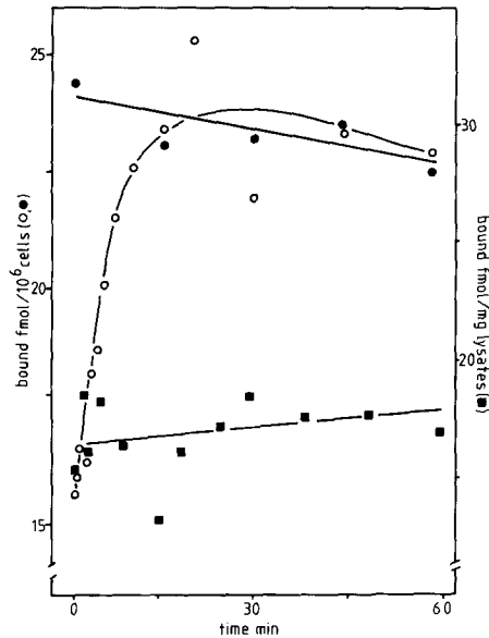
FIGURE 2 Kinetics of reappearance of [ ^3\text{H} ]CGP-12177 binding sites at 37^\circ\text{C} . Isoproterenol-treated cells (O), control cells (●), or cells that were lysed after isoproterenol treatment (■) were incubated with 3 nM [ ^3\text{H} ]CGP-12177 at 37^\circ\text{C} for the times indicated, chilled, and incubated for a further 24 h at 4^\circ\text{C} . For intact cells the amount of bound ligand is given as femtomole per 10^6 cells; for lysates it is given as femtomole per milligram protein.
