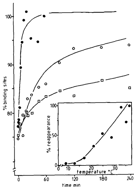
FIGURE 3 Temperature dependence of the reappearance of [ ^3\text{H} ]CGP-12177 binding sites. After isoproterenol pretreatment, cells were incubated at different temperatures. In each experiment the total number of binding sites was determined after 60 min at 37^\circ\text{C} . The data from the single experiments were normalized to that value (mean \pm SE; n = 6 ). The data are shown for 33^\circ\text{C} (●), 21^\circ\text{C} (○), and 13^\circ\text{C} (□). (inset) Temperature dependence of reappearance of CGP-12177 binding sites after 15 min. Percentage of reappearance of binding sites after 15 min was calculated and plotted as a function of temperature. The difference between the number of binding sites at 0- and at 60-min incubation at 37^\circ\text{C} was set arbitrarily at 100%. The temperature dependence of the kinetics has been determined as described above.
