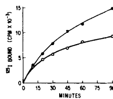
FIGURE 3 Effect of ligand concentration on thermal activation. ^{125}\text{I} -LRSC stock ( 14.2 \mu\text{g/ml} ) was heated at 37^\circ\text{C} for 30 min and then diluted into binding buffer to 12.7 \text{ ng/ml} (○). ^{125}\text{I} -LRSC stock was diluted to 12.7 \text{ ng/ml} with binding buffer and then heated at 37^\circ\text{C} for 30 min (●).
