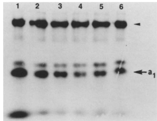
FIGURE 3 Fluorograph of pulse-labeled medium collagens. Collagen was isolated from [ ^3\text{H} ]proline-labeled media from days 0-2 (1), 2-4 (2), 4-7 (3), 7-9 (4), 9-11 (5), and 11-14 (6). The collagens were electrophoresed under nonreducing conditions on a 5% gel. The arrowhead indicates the position where Type III collagen migrates on this gel.
