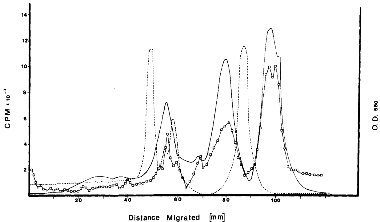
FIGURE 2 Cyanogen bromide digest of [ ^3\text{H} ]proline-labeled cell-layer collagens. The long-term labeled cell-associated matrix collagen was subjected to CNBr digest in the presence of bovine Type II collagen; Type I collagen was digested in a companion tube. The peptides were electrophoresed on a 7.5% gel and stained before scanning and slicing for counting. Unlabeled Type I peptide (dashed line), unlabeled Type II peptides (straight line), labeled peptides from cell layer ( \square ).
