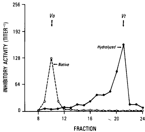
FIGURE 5 Chromatography of alkaline hydrolyzed (●—●) or untreated native (○---○) intestinal mucin on Sepharose 4B. V_0 , void volume. V_t , included volume.
