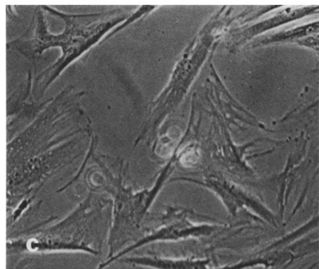
FIGURE 3 Human skin fibroblasts labeled with dil and viewed at low magnification. (a) TIRF. \theta = 72.5^\circ ; d = 120 nm. (b) Epifluorescence of the same field. The variable fluorescence from cell to cell is characteristic of dil labeling. The somewhat mottled intensity and interference fringe pattern is a result of the coherence of the laser illumination. (c) Phase contrast of the same field. A \times 10 phase-
