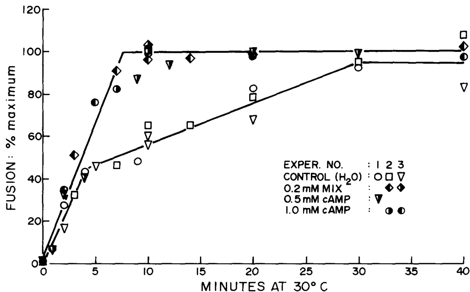
FIGURE 1 Effects of MIX and cAMP on the vacuole fusion reaction in Rv-containing homogenates prepared from stationary phase cells. The figure shows the pattern of fusion reaction in the controls (open symbols), and after the addition of 0.2 mM MIX (half-filled diamonds), 0.5 mM cAMP (half-filled triangles), and 1 mM cAMP (half-filled circles). Fusion (%F) was measured as described in Materials and Methods, and the results are plotted relative to the maximum amount of fusion obtained in each experiment (plateau level = 100%).
