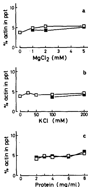
FIGURE 7 Effects of the concentration of MgCl 2 ( a ), KCl ( b ), and protein ( c ) on polymerization of the actin harvested from the D - subline. CM-treated D - , ■. Untreated D - , □.
