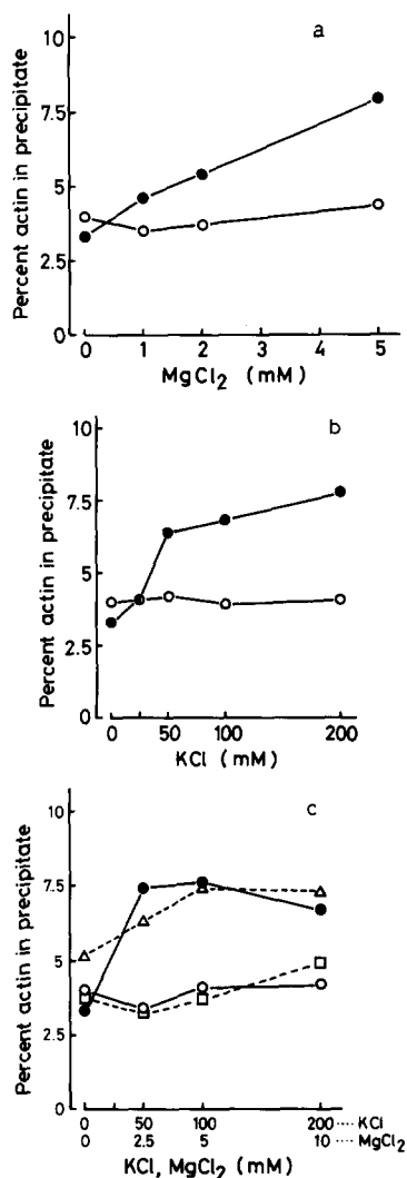
FIGURE 6 Effects of the salt concentration on actin polymerization. In a , b , and c , the protein concentration of the crude cell extract was adjusted to 4 mg/ml with 0.34 M sucrose buffer and combined with salt solution to give the final concentration indicated in the figure. The mixtures were incubated at 30°C for 1.5 h, then centrifuged at 100,000 g for 2.5 h at 25°C. The pellet was dissolved in depolymerizing buffer, ultrasonicated, and the mixture was used for electrophoresis. Ordinate: counts in actin band/total counts in the pellets applied to gel electrophoresis. Abscissa: final concentration of salts. CM-treated M1 cells, ●. Untreated M1 cells, ○. Untreated D - subline, □. Untreated Mml subline, △.
