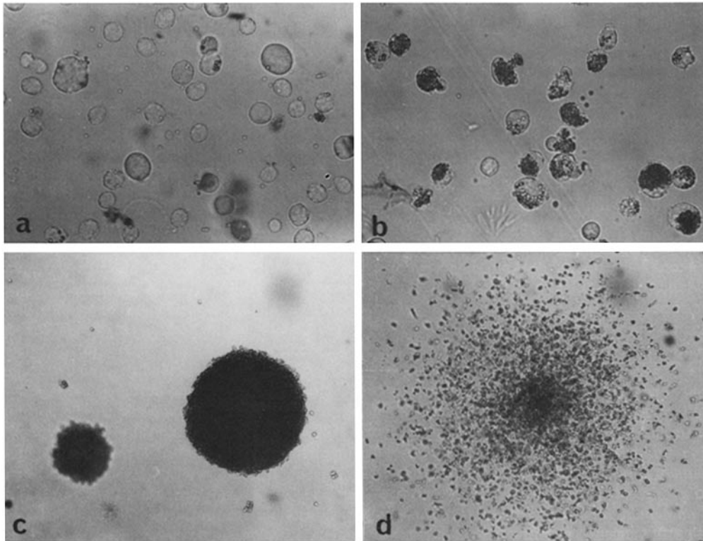
FIGURE 1 Tests for phagocytosis (a and b) and cell motility (c and d). The MI control cells are shown in a and c. Cells differentiated by incubation with CM for 2 d are shown in b and d. (a and b) \times 400 . (c and d) \times 50 .
