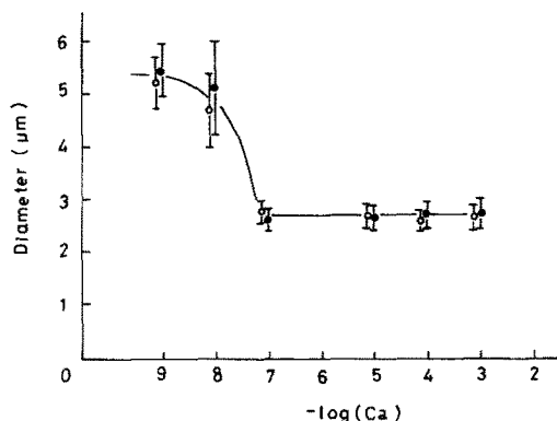
FIGURE 5 Ca dependence of the helical diameter of the DMT. Ca concentrations <10^{-7} M were controlled by a changing ratio of CaCl 2 and MgSO 4 to EGTA (1 mM) in medium containing 20 mM Tris-HCl buffer (pH 8.0). Concentrations >10^{-6} M were obtained by simple addition of CaCl 2 to 20 mM Tris-HCl buffer solution (pH 8.0).
