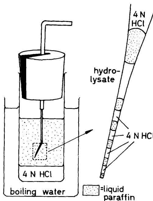
FIGURE 1 Illustration of the procedure for quantitative hydrolysis of RNA in amounts down to 100 to 1000 \mu\mu\text{g} .
