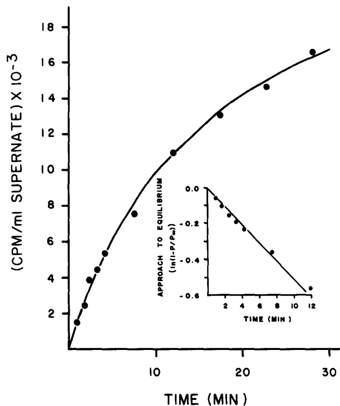
FIGURE 3 The time course of ^{42}\text{K} efflux across rabbit PMN membranes. Inset represents the same data in a semilogarithmic plot. P and P_{\infty} , respectively, refer to the counts per minute per milliliter of supernate at any given time and at equilibrium.
