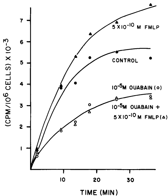
FIGURE 10 Effect of FMLP and ouabain on the time course of 42 K influx across rabbit PMN membranes. Ouabain and/or FMLP were added at zero time. Each point represents the mean of duplicate determinations.
