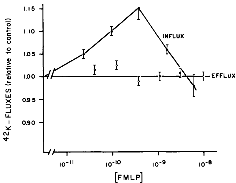
FIGURE 9 Effect of varying concentrations of FMLP on 42 K fluxes. Each point represents the mean of quadruplicate determinations and the vertical bars represent the standard error of the mean.
