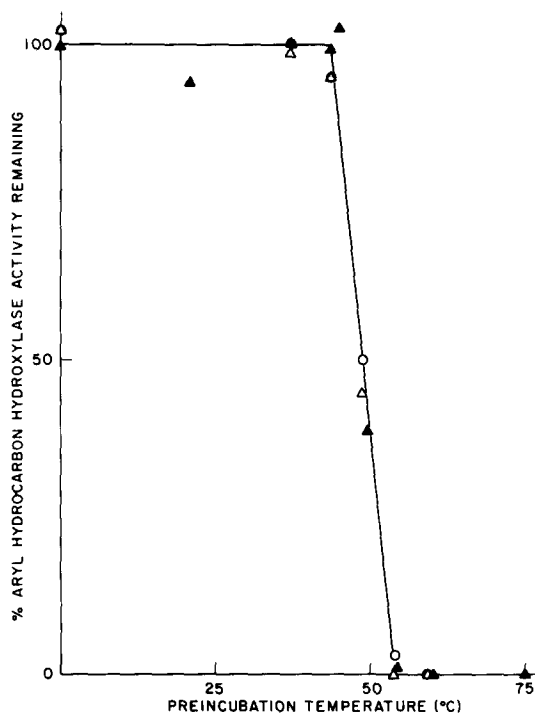
FIGURE 3 Heat stability of benz[a]anthracene-induced aryl hydrocarbon hydroxylase in heteroploid parental cells and subclones. Cells were exposed to benz[a]anthracene (1 \mu\text{g/ml} ) for 8 h. Cell homogenates were preincubated for 5 min without NADPH or substrate. The standard incubation followed the preliminary incubation. ▲, parents; ○, subclone 1; △, subclone 2.
