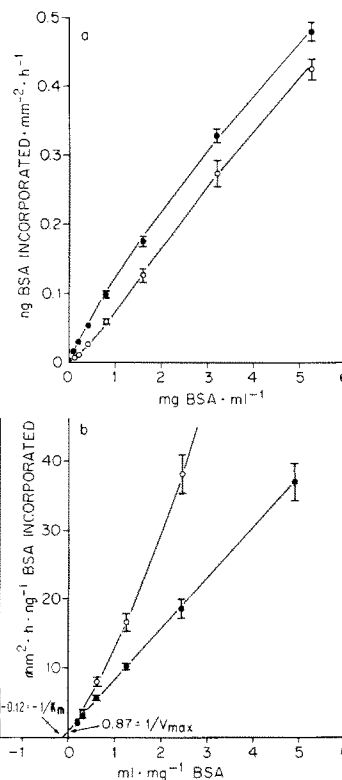
FIGURE 5 [ ^{14}\text{C} ]BSA incorporation by oocytes as a function of concentration in both the absence (open circles) and the presence (closed circles) of 10 \text{ mg} \cdot \text{ml}^{-1} vitellogenin. Normal ( a ) and double-reciprocal ( b ) plots are provided. Each point represents the average value derived from 12 oocytes, and the range bars indicate s . The straight line drawn in ( b ) for [ ^{14}\text{C} ]BSA incorporation in the presence of vitellogenin represents the least-squares fit to the points.
