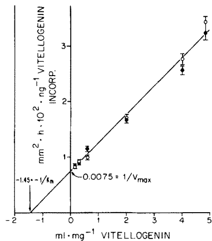
FIGURE 3 [ ^{14}\text{C} ]Vitellogenin incorporation by oocytes as a function of concentration, in both the absence (open circles) and the presence (closed circles) of 10 \text{ mg} \cdot \text{ml}^{-1} BSA. The line represents the least-squares fit to all the points. Each point represents the average value derived from 12 oocytes, and the range bars indicate s . Double-reciprocal plot.
