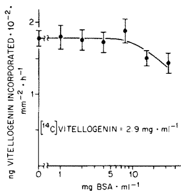
FIGURE 4 Relative incorporation of [ ^{14}\text{C} ]vitellogenin as a function of BSA concentration. The concentration of [ ^{14}\text{C} ]vitellogenin was held constant at 2.9 \text{ mg} \cdot \text{ml}^{-1} . Each point represents the average value derived from eight oocytes, and the range bars indicate s . Semilog plot.
