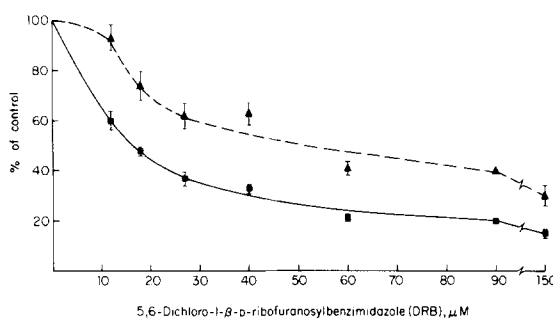
FIGURE 3 Effects DRB on nucleoplasmic and nucleolar RNA synthesis in L cells. L cells from monolayer cultures were grown for 2 days in suspension culture in spinner modification of MEM with 7% fetal calf serum. Initial cell concentration was 2 \times 10^6 cells/ml, and the vol was in the range of 200 ml. The cell concentration was maintained between 2 and 4 \times 10^5 cells/ml by daily dilution. The harvested cells were washed once with warm medium and distributed among six aliquots of 50 ml each containing 4 \times 10^5 cells/ml ( 2 \times 10^7 aliquot). Cells were incubated at 37°C for 15 min in serum-free MEM or in medium containing DRB at varying concentrations. [ 3 H]Uridine, 15 μCi/ml, was then added for a pulse of 15 min. After labeling, the cells were harvested on ice, collected by centrifugation, and washed once with PBS. The nuclei and then the nucleoplasmic and nucleolar fractions were isolated as described in Materials and Methods. Incorporation of [ 3 H]uridine into acid-precipitable material in the nucleoplasmic and nucleolar fractions was determined. Results of 12 experiments are shown. In the untreated controls, the mean radioactivity in the nucleoplasmic fraction was 974,100 cpm and in the nucleolar fraction it was 598,300 cpm. (■—■), Nucleoplasmic fraction; (▲---▲), nucleolar fraction. The vertical bars indicate probable error for data points. Results of a single experiment are given for 90 μM DRB.
