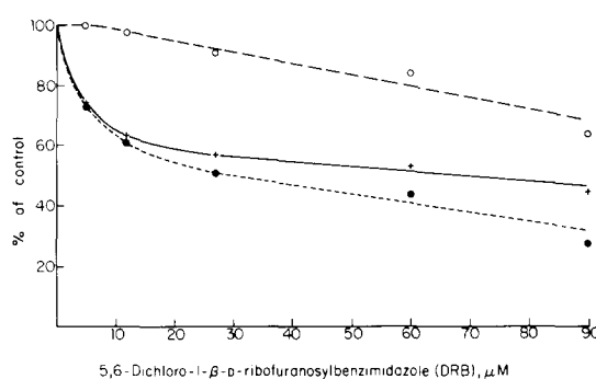
FIGURE 1 Relation between concentration of DRB and effects on [ ^3\text{H} ]uridine uptake and RNA synthesis in L cells. L cells were planted in 60-mm plastic petri dishes at a concentration of 2.5 \times 10^6 cells/plate in Eagle's MEM with 5% fetal calf serum. 24 h later, the incomplete monolayers of L cells were washed once with warm Eagle's medium and incubated at 37°C for 15 min with DRB at varying concentrations in serum-free MEM, 5 ml/plate. Controls received no DRB. Three dishes were used per variable. The cultures were then pulse-labeled for 15 min with [ ^3\text{H} ]uridine added in a vol of 100 \mu\text{l} to give 2.5 \mu\text{Ci/ml} . In the DRB-treated cultures the compound remained present during the pulse. After the pulse, the medium was aspirated and the dishes were washed and frozen. Subsequently, 1 ml of distilled water was added per dish and the cells scraped off with a silicone square. The plates then received 1 ml of 10% TCA. Two aliquots of 10 \mu\text{l} each were used for determination of total cell-associated radioactivity. The remainder was used to measure acid-precipitable radioactivity. To determine the effect of DRB on RNA synthesis, the acid-precipitable cpm were corrected for effect of DRB on uptake of [ ^3\text{H} ]uridine into cells as described in Materials and Methods. Mean results of two experiments are shown. In the untreated controls, the total radioactivity was 83,053 cpm and the acid-precipitable radioactivity was 5,976 cpm. (O---O), Total cellular uptake of [ ^3\text{H} ]uridine; (+---+), RNA synthesis; (●---●), incorporation of [ ^3\text{H} ]uridine into acid-precipitable material.
