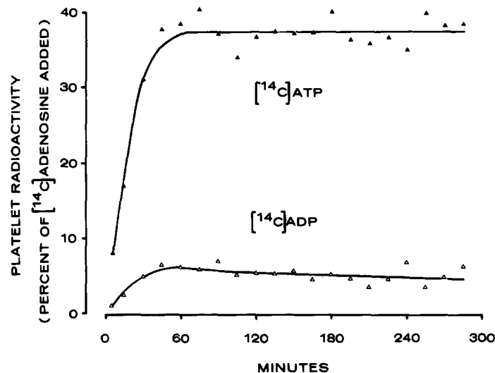
FIGURE 4 Percentages of ^{14}\text{C} as [^{14}\text{C}]\text{ATP} and [^{14}\text{C}]\text{ADP} within platelets at various times after addition of [^{14}\text{C}]\text{adenosine} . At the times indicated, aliquots of the platelet suspension were removed and extracted with perchloric acid. The radioactive ATP and ADP in the perchloric acid extracts were separated by paper chromatography and counted. Results were expressed as percentages of the counts per minute added to the platelet suspension. (Appropriate corrections were made for small amounts of [^{14}\text{C}]\text{ATP} and [^{14}\text{C}]\text{ADP} in the supernate of the platelet suspension.) The suspension contained 184,000 cpm/ml. The platelet count was 10^6/\mu\text{l} .
