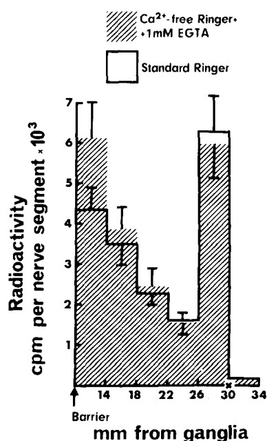
FIGURE 1 The effect of Ca 2+ -free Ringer's, containing 1 mM EGTA, on the transport of [ 3 H]leucine-labeled TCA-insoluble material in the sciatic nerve. The preparations were incubated for 17 h at 18°C. The two preparations from the same animal were used, one serving as a control and the other as a test preparation. Compartment A contained 10 \mu Ci [ 3 H]leucine (38 Ci/mmol) in 1 ml standard Ringer's. Compartments B and C of the control were perfused with standard Ringer's and of the test preparation with Ca 2+ -free Ringer's. The Ca 2+ -free Ringer's contained 1 mM EGTA. The position of the ligature is shown (X). Each bar represents the mean of 17 experiments. The vertical lines indicate the SEM.
