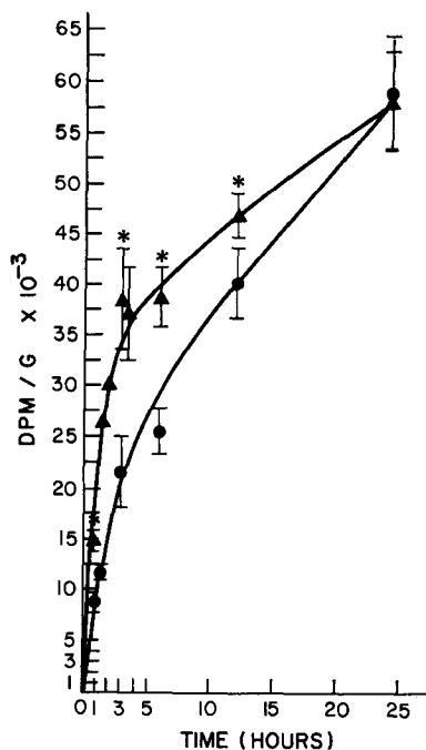
FIGURE 1 Effect of pilocarpine on the incorporation of [ ^3\text{H} ]myoinositol into the lipids of the pancreas. Pilocarpine and [ ^3\text{H} ]myoinositol were injected at zero time, as described under Materials and Methods. The triangles are the lipid radioactivity from pancreases of guinea pigs injected with pilocarpine. The circles are the lipid radioactivity from unstimulated animals. The values are given as the means \pm the standard error of the mean. The asterisks indicate that the differences between the unstimulated and stimulated values were significant at the P < 0.001 level, as determined by the t test.
