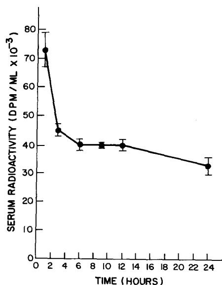
FIGURE 5 The radioactivity in guinea pig serum after injection of [2\text{-}^3\text{H}] myo-inositol. The vertical bars represent the standard error of the mean. The radioactivity in the serum was determined, as described under Materials and Methods.
