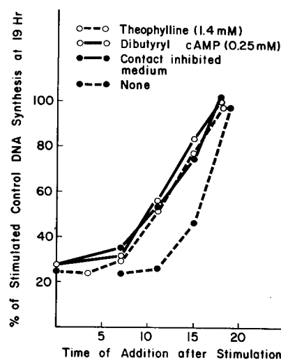
FIGURE 8 Kinetics of irreversible commitment to DNA synthesis. Four groups of confluent cultures were refeed with EMEM containing 10% serum. DNA synthesis in one group was followed as a function of time after stimulation (●---●). The synthesis in this group at 19 hr served as the control value. At the times after stimulation indicated on the abscissa, cultures in the other three groups were refeed with contact-inhibited medium or with fresh medium containing either 1.4 mM theophylline or 0.25 mM db-cAMP. DNA synthesis for all cultures in these three groups was determined 19 hr after the initial stimulation and plotted as a function of the time at which one of the inhibitory media was added to the stimulated cultures. All levels of synthesis are expressed as a percentage of the synthesis in the control group at 19 hr. Each point is the average of two determinations.
