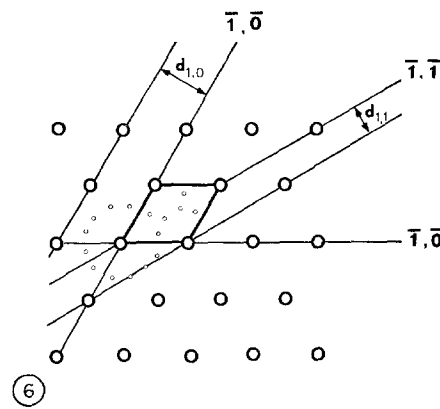
FIGURE 6 Schematic representation of the crayfish myofilament array. The large circles represent the myosin filaments. These filaments lie in planes, forming a lattice with the distances between the lattice planes indicated. The small circles represent the actin filaments, 12 of which are arranged more or less equidistant around each thick filament (shown completely for one thick filament and partially for three others). The heavy solid lines delineate the unit cell, containing one thick filament ( \frac{1}{6} + \frac{2}{6} + \frac{1}{6} + \frac{2}{6} of the included thick filaments) and six thin filaments. This results in a 1:6 unit-cell ratio of thick filaments to thin.
