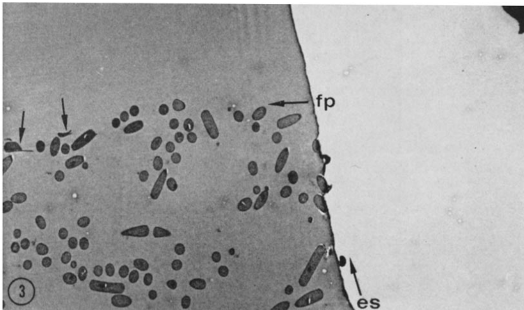
FIGURE 3 Freeze-fractured and subsequently embedded and sectioned bacteria. Note edge of thin section (es), fracture plane (fp), and freeze-fractured bacteria (arrows). \times 45,000 .
