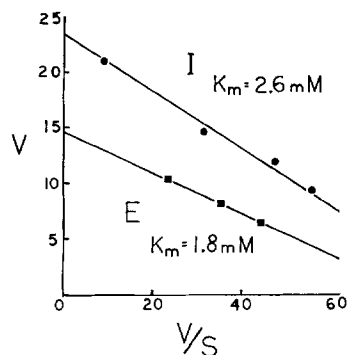
FIGURE 4 Kinetic plot of the effect of GABA concentration on transaminase activity in single E- and I-axon homogenates. The velocity ( V ) is expressed as moles \times 10^{11} /hr. For experimental details see text, Methods, and reference 13. The apparent K_m 's in the E- and I-axon homogenates are not significantly different.
