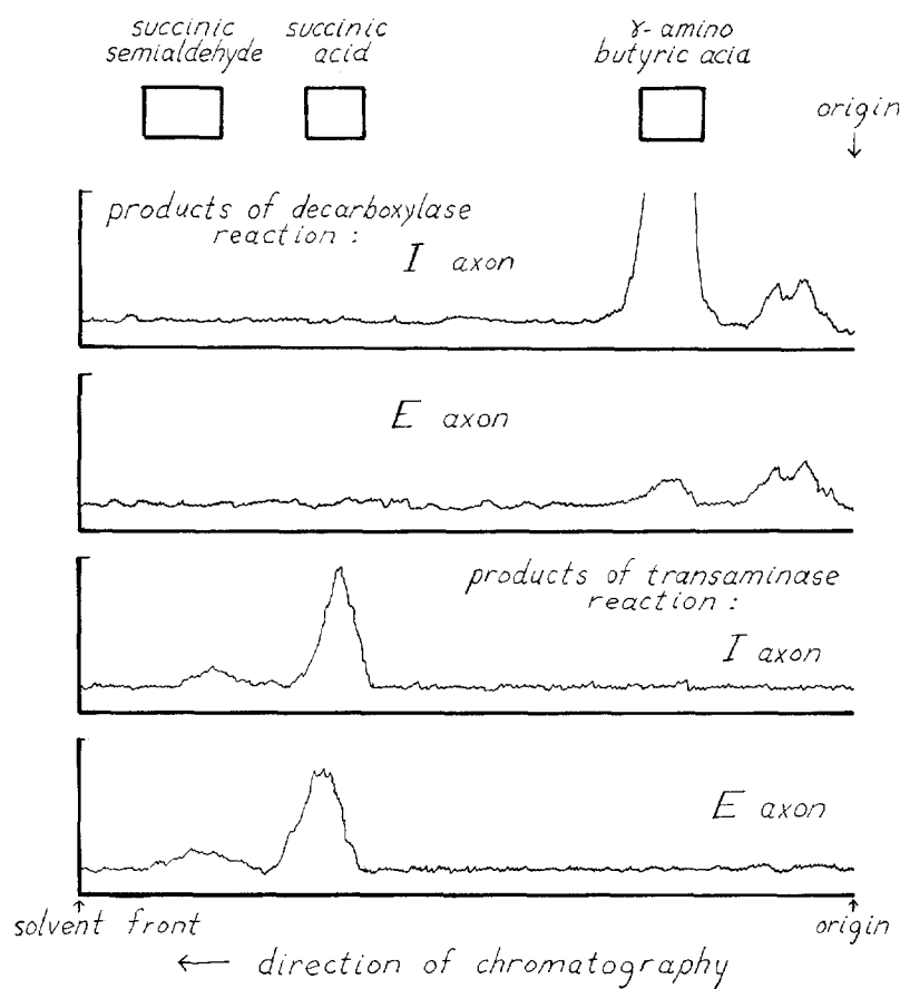
FIGURE 3 Scans of radioactivity in chromatograms of reaction products of decarboxylase and transaminase reactions. The double peak near the origin in decarboxylase incubations is also seen in boiled enzyme controls and is a contaminant. The principal product formed in both E- and I-axon decarboxylase incubations corresponds to GABA. There are no radioactive contaminants seen in controls of transaminase incubations, and the products formed correspond to succinate and succinic semialdehyde. Paper chromatography was ascending at room temperature and solvent 2 was used for decarboxylase products and solvent 3 for transaminase products. See Methods for experimental details. Full scale (indicated by bar) was 500 cpm.
