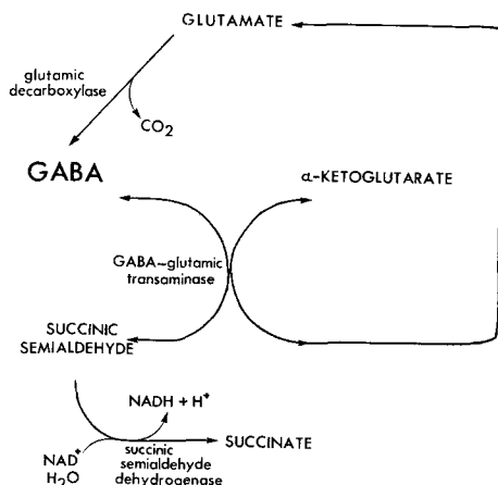
FIGURE 1 The pathway of GABA metabolism in the lobster nervous system.
