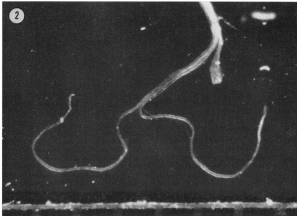
FIGURE 2 Single axons dissected from the meropodite segment of the walking leg of the lobster, as viewed through a dissecting microscope. The ruler divisions are 1 mm and individual axons are 40–50 \mu in diameter. Axons are identified by stimulation. A knot is tied in one axon (the E in this case) to facilitate identification in case of axon damage during the dissection. About 5–6 cm lengths of axon are routinely obtained (see reference 5 and Methods for details).
