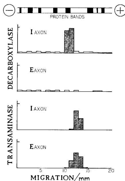
FIGURE 5 Decarboxylase and transaminase enzyme activities measured in slices of micropolyacrylamide gel columns. The experimental procedure is described in Methods. The gel pattern illustrated at the top is a typical distribution of protein bands seen on inspection after conjugation of proteins with fluorescent dansyl reagent. No significant differences were noted between E- and I-axons, and it was not possible to associate particular bands with specific enzymes. Full scale (indicated by bar) was 400 cpm.
