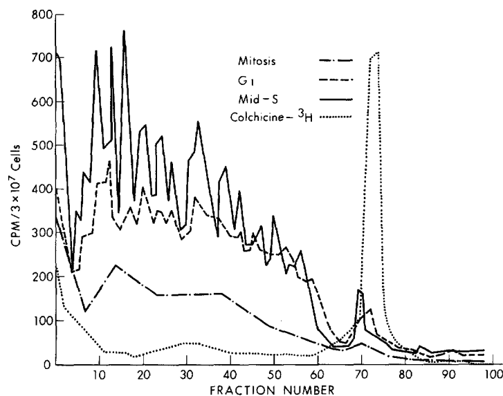
FIGURE 1 Acrylamide gel electropherogram of 100,000 g supernate from HeLa cells in G_1 , mid-S, and mitosis pulsed with leucine- ^{14}C and then labeled in vitro with colchicine- ^3H . Only the colchicine label from the G_1 sample is shown. The colchicine label from the S sample was similarly exactly superimposed on the most rapidly migrating leucine peak but is not plotted, to avoid confusion.
