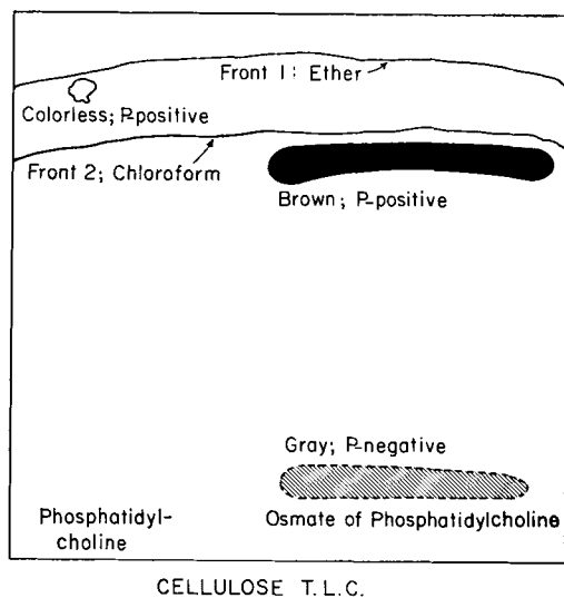
CELLULOSE T.L.C. FIGURE 1 Thin-layer chromatogram of the methanol-soluble osmium derivative of di-11-octadecenoyl phosphatidylcholine. The osmium derivative and a sample of the unreacted phospholipid were applied in narrow bands. The plate was developed first with diethyl ether, then air-dried, and redeveloped with chloroform. The unreacted phospholipid migrated with the ether front, while the osmium derivative remained at the origin. In chloroform the osmium derivative migrated with the front, leaving a faint gray, phosphorus-negative band at the origin. The brown band at the chloroform front was phosphorus-positive and osmium-positive.
