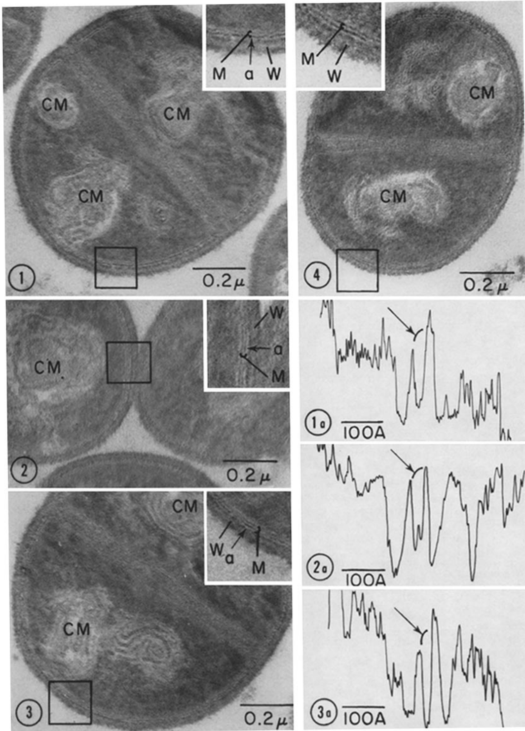
FIGURES 1 through 4 Sections of Staphyococcus aureus cells cultivated on agar for 5 hr and fixed in osmium tetroxide for 18 hr. Figs. 1, 2, and 3, \times 80,000 ; Fig. 4, \times 70,000 . The regions within the squares are enlarged (insets). The outermost two dark layers and the intervening light layer are attributed to the cell wall ( W ). The plasma membrane ( M ) and the cytoplasmic membranous structure ( CM ) show the unit membrane structure. Insets 1, 2, and 3, \times 130,000 ; Inset 4, \times 180,000 .
