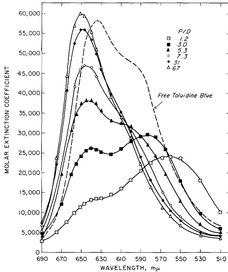
FIGURE 1 Spectra of free TB, 1.7 \times 10^{-5} M, and of TB bound to native DNA at various P/D values. The nitrogen and sulfur content of samples of purified toluidine blue was used to determine E_m of the free dye at 635 \text{ m}\mu as a function of concentration. Thus, the number of moles of dye at the beginning of each titration was determined from the optical density at 635 \text{ m}\mu , and was used to convert the spectrum of bound dye at any P/D from optical density to molar extinction.
