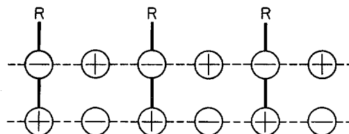
FIGURE 1 Model of a tricomplex system of phospholipid amphions, microcations, and microanions. R represents the apolar part of the lipid molecules.
