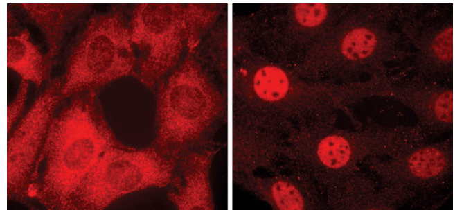
MAL (red) nuclear export (left) is prevented in serum-stimulated cells (right) by the loss of G actin binding.
