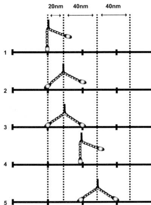
Figure 10. The relationship between the double step events and hypothetical states in the walking cycle of a double-headed myosin V molecule. In this model, a myosin V molecule walks from left to right along an actin filament (solid lines). The helical repeat of actin is indicated by tick marks, and dashed lines indicate 20- and 40-nm displacements from the site of initial attachment. After attachment, the myosin V molecule undergoes its working stroke (states 1–2) with the attachment of the second head following very rapidly (state 3). The working stroke and double-headed attachment results in the low variance first step. After the second head's powerstroke, release of the rear head discharges the intramolecular strain, bringing the rear head toward the next actin-binding site. Under normal processive movement, myosin V would then bind to the next actin-binding site (states 3–5), thus giving rise to the 40-nm walking stride. However, the expressed M5_{HMM} did not demonstrate processivity but stalled during its second step at an intermediate displacement level, having high position variance (state 4) resulting from single-headed attachment.
