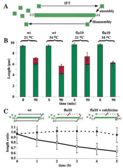
Figure 5. Role of IFT in flagellar maintenance. (A) Model: IFT particles carry structural proteins, including tubulin, to the plus end of the flagellum where they are incorporated in order to compensate for subunits removed during the disassembly portion of the turnover process. Plus and minus ends of the flagellar outer doublet microtubules are indicated by (+) and (-). (B) fla10 mutants at the nonpermissive temperature block the assembly portion of turnover, as judged by the lack of tagged tubulin incorporation at the tip, but do not block disassembly, as judged by shortening of the unlabeled region of the flagella. This confirms that IFT is needed for ongoing incorporation of new tubulin at the distal end. Average number of measurements per graph entry was 19. (C) Colchicine is predicted to rescue the fla10 phenotype by blocking outer doublet disassembly. As shown in graph, colchicine blocks flagellar resorption in fla10 cells shifted to the nonpermissive temperature. (Dotted line) fla10 cells treated with 3 mg/ml colchicine. (Solid line) Untreated fla10 cells. Length ratio plots ratio of length at nonpermissive temperature to length at permissive temperature.
