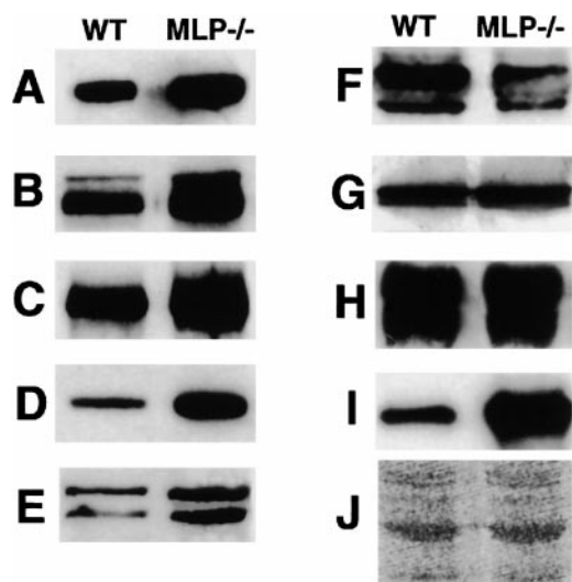
Figure 3. Expression levels of intercalated disk proteins are changed in adult MLP^{-/-} hearts. Immunoblots on whole heart muscle samples of wild-type (WT) or MLP^{-/-} mice with antibodies against cadherin (A), \beta -catenin (B), plakoglobin (C), \alpha -catenin (D), vinculin (E), connexin-43 (F), desmoplakin (G), desmoglein (H), and N-RAP (I). J shows a part of a Ponceau-stained filter. Adherens junction-associated proteins appear upregulated (A–E, and H); the gap junction component connexin-43 seems downregulated (F), and the expression levels of the desmosomal markers desmoplakin and desmoglein are unaffected (G). Representative blots with extracts from one animal per lane are shown.
